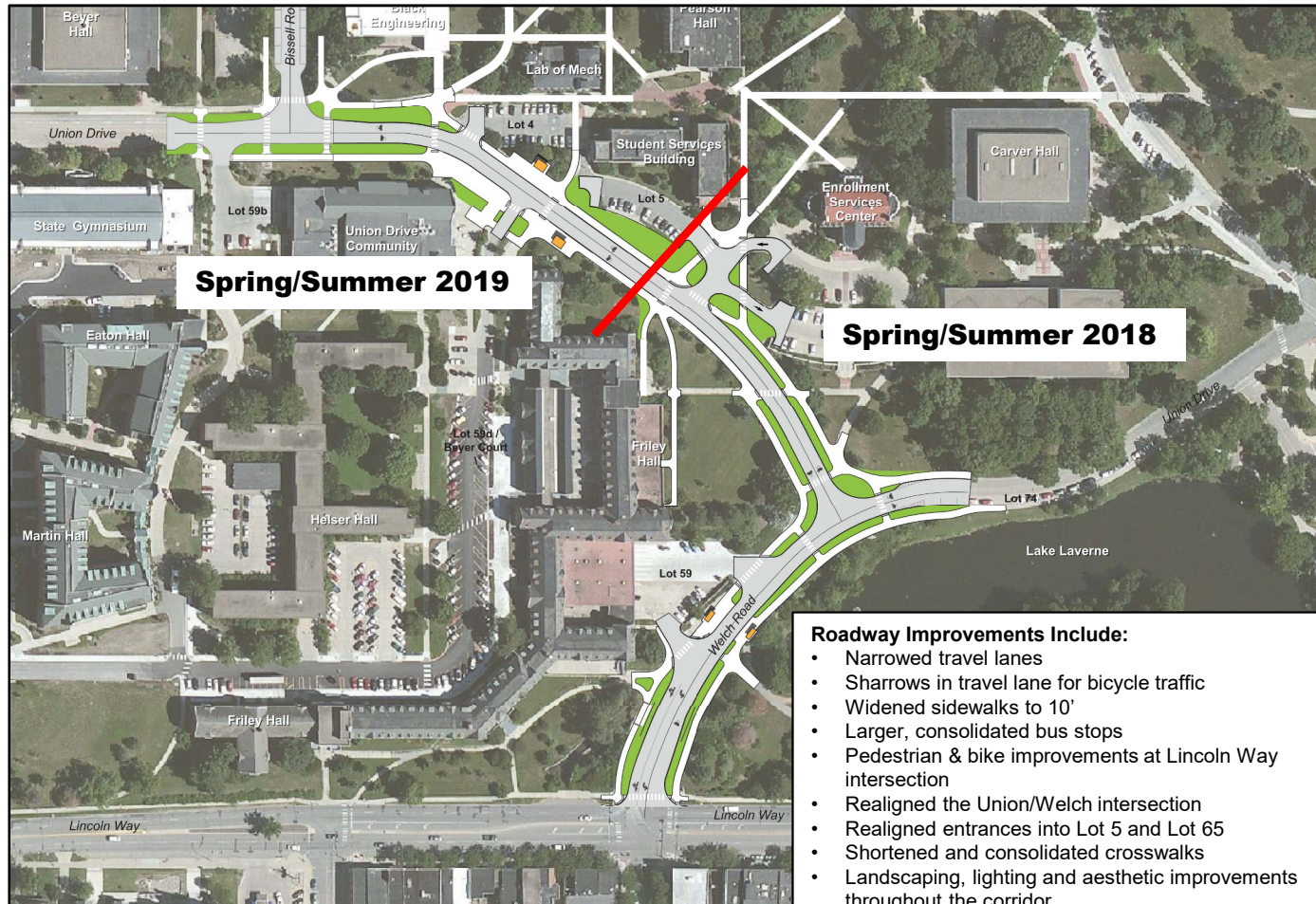
CONCEPT PLAN
